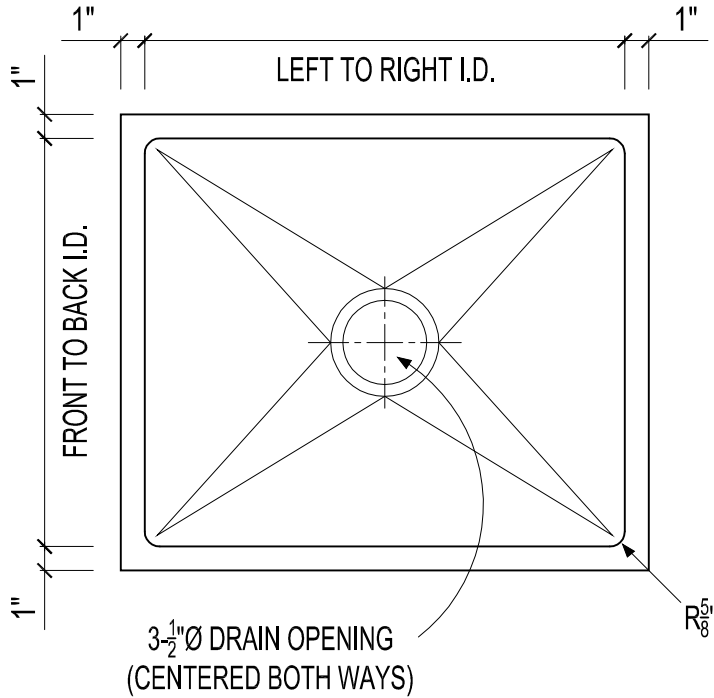
PLAN VIEW
